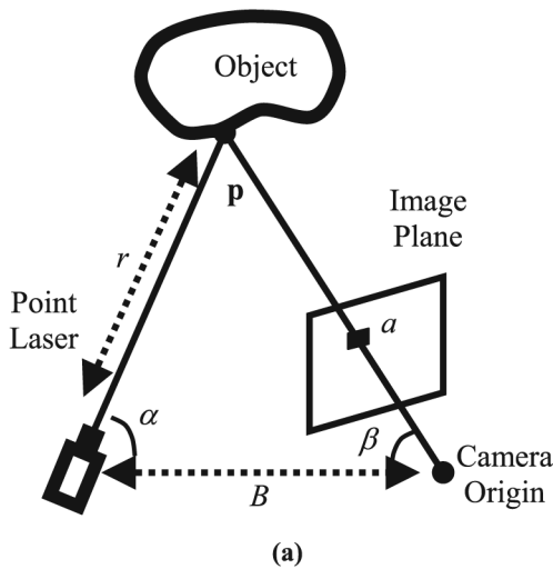
Figure 2 Structured light system. (a) Diagram for principles of operation. The laser illuminates point p and projects to pixel a . (b) A sheet-of-light example. The laser stripe across the objects projects to the image plane of the camera such that it illuminates only 1 pixel in each image column
